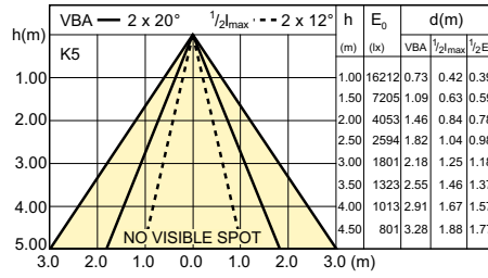
Beam diagram - MASTER CDM-R111 Elite 70W/930 GX8.5 24D
